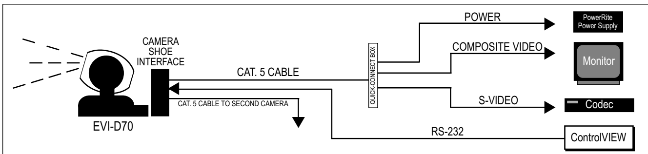
Figure 2 – EZCamera cable system with a quick-connect box.
